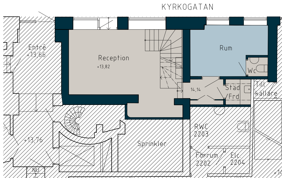
PLAN 2, GATUPLAN
