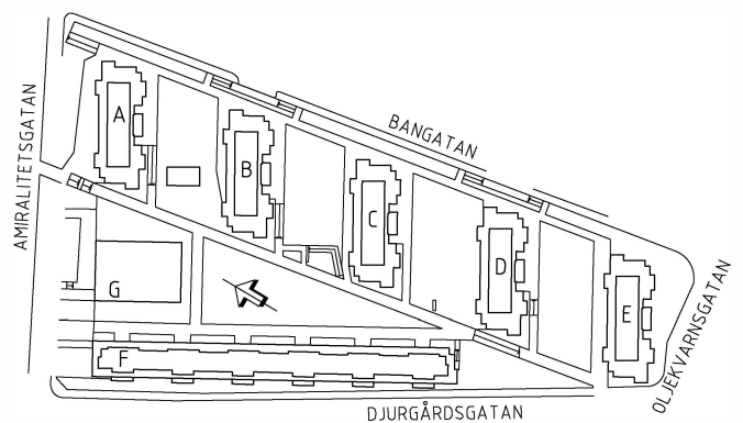
Orienteringsplan
